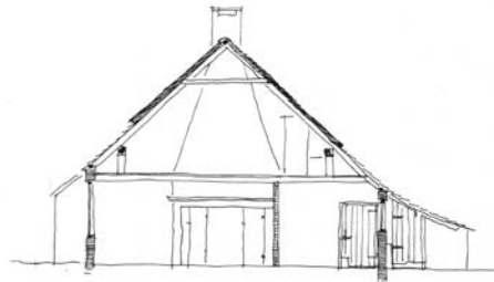
DOORSNED E OVER DE HERD.
